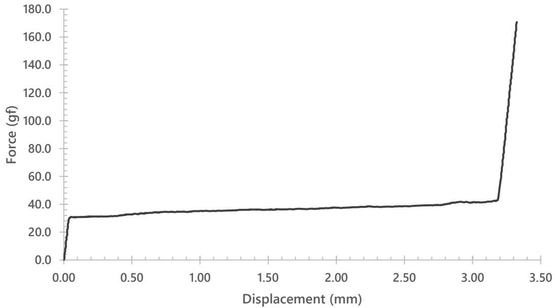
Gateron Magnetic Jade Ultra (Upstroke)
